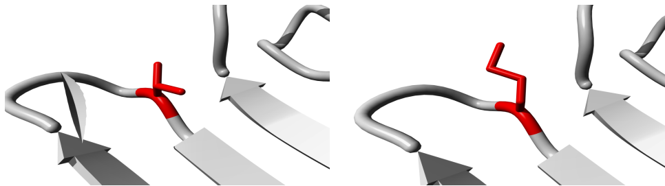
Figure 2.13: Molecular visualization of the WT (left) and variant (right) amino acid. The residues colored in red represents the wild type (VAL) and variant residue (MET).
