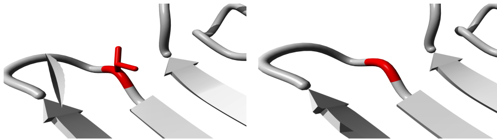
Figure 2.13: Molecular visualization of the WT (left) and variant (right) amino acid. The residues colored in red represents the wild type (VAL) and variant residue (GLY).
