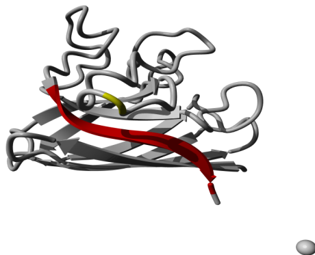
Figure 2.4: Molecular visualisation of TANGO aggregation-prone regions. This molecular image shows the TANGO aggregation-prone regions as red colored segments. The structural location of the variant residue is colored in yellow.
