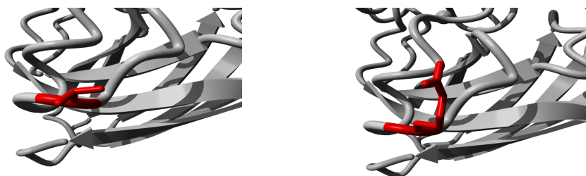
Figure 2.13: Molecular visualization of the WT (left) and variant (right) amino acid. The residues colored in red represent the wild type (THR) and variant residue (ARG).
