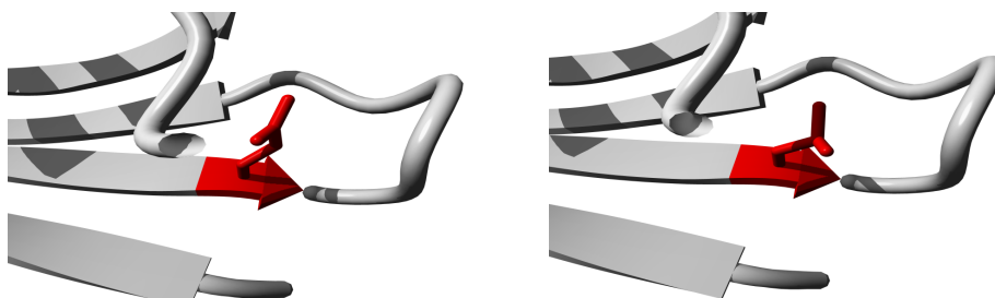
Figure 2.13: Molecular visualization of the WT (left) and variant (right) amino acid. The residues colored in red represents the wild type (GLN) and variant residue (LEU).
