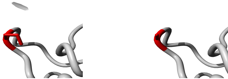
Figure 2.13: Molecular visualization of the WT (left) and variant (right) amino acid. The residues colored in red represents the wild type (PRO) and variant residue (ALA).
