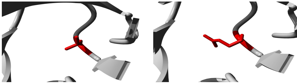
Figure 2.13: Molecular visualization of the WT (left) and variant (right) amino acid. The residues colored in red represents the wild type (LEU) and variant residue (ARG).
