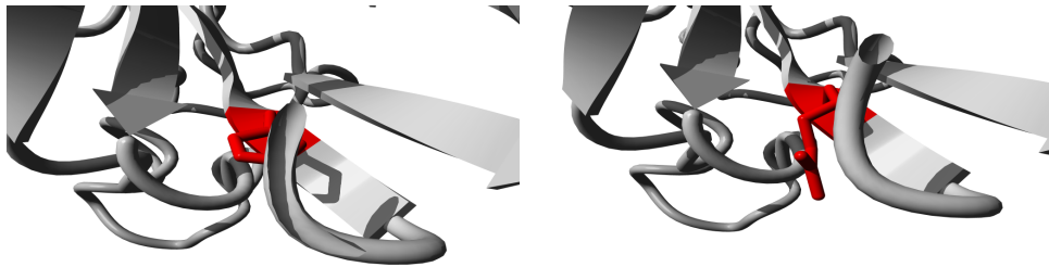
Figure 2.13: Molecular visualization of the WT (left) and variant (right) amino acid. The residues colored in red represents the wild type (HIS) and variant residue (ARG).
