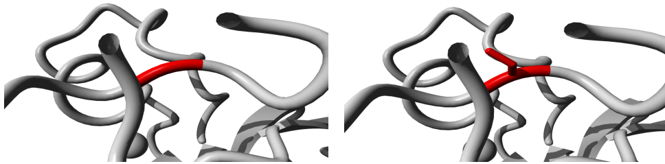
Figure 2.13: Molecular visualization of the WT (left) and variant (right) amino acid. The residues colored in red represents the wild type (GLY) and variant residue (SER).
