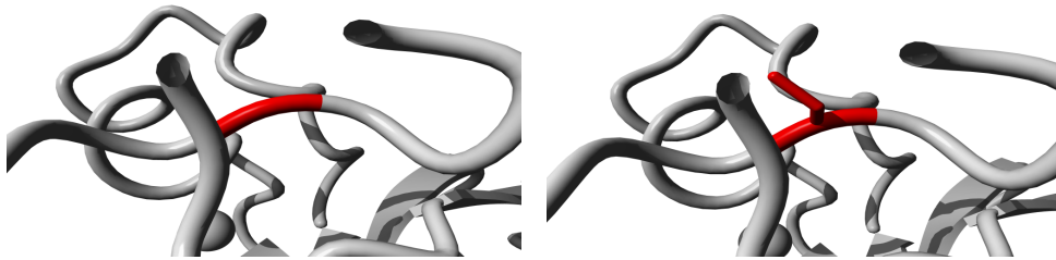
Figure 2.13: Molecular visualization of the WT (left) and variant (right) amino acid. The residues colored in red represents the wild type (GLY) and variant residue (CYS).
