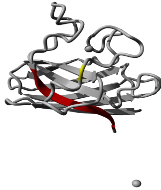
Figure 2.4: Molecular visualisation of TANGO aggregation-prone regions. This molecular image shows the TANGO aggregation-prone regions as red colored segments. The structural location of the variant residue is colored in yellow.
