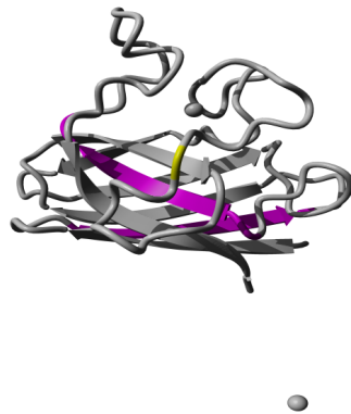
Figure 2.12: Molecular visualisation of LIMBO chaperone-binding sites. This molecular image shows the LIMBO chaperone-binding sites as pink colored segments. The structural location of the variant residue is colored in yellow.
