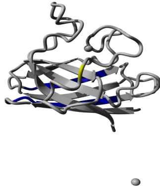
Figure 2.8: Molecular visualisation of WALTZ amyloid-forming regions. This molecular image shows the WALTZ aggregation-prone regions as blue colored segments. The structural location of the variant residue is colored in yellow.
