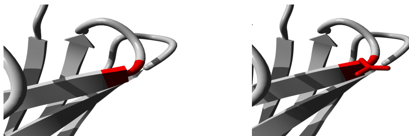
Figure 2.13: Molecular visualization of the WT (left) and variant (right) amino acid. The residues colored in red represents the wild type (GLY) and variant residue (ASP).
