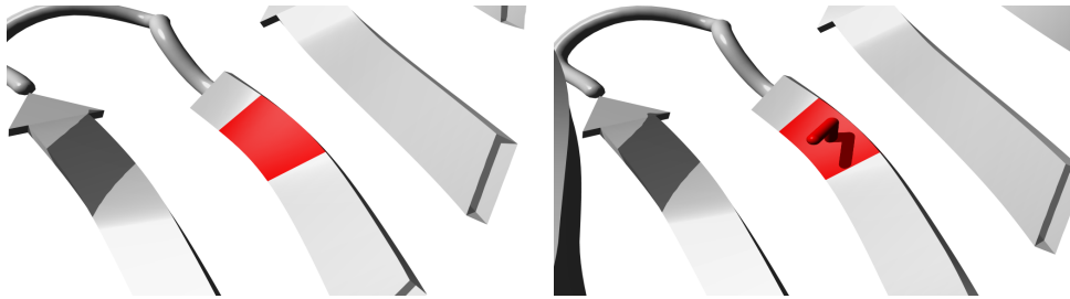
Figure 2.13: Molecular visualization of the WT (left) and variant (right) amino acid. The residues colored in red represents the wild type (GLY) and variant residue (SER).
