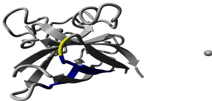
Figure 2.8: Molecular visualisation of WALTZ amyloid-forming regions. This molecular image shows the WALTZ aggregation-prone regions as blue colored segments. The structural location of the variant residue is colored in yellow.
