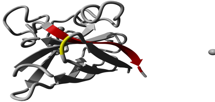
Figure 2.4: Molecular visualisation of TANGO aggregation-prone regions. This molecular image shows the TANGO aggregation-prone regions as red colored segments. The structural location of the variant residue is colored in yellow.
