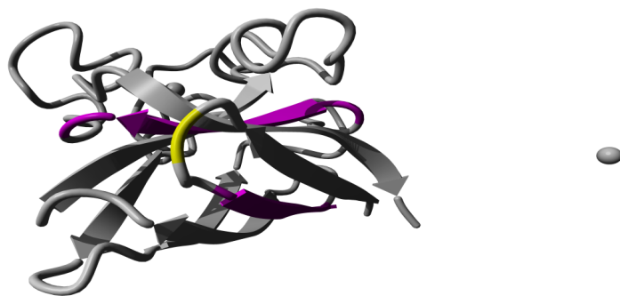
Figure 2.12: Molecular visualisation of LIMBO chaperone-binding sites. This molecular image shows the LIMBO chaperone-binding sites as pink colored segments. The structural location of the variant residue is colored in yellow.
