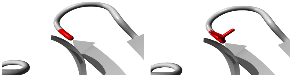
Figure 2.13: Molecular visualization of the WT (left) and variant (right) amino acid. The residues colored in red represents the wild type (GLY) and variant residue (VAL).
