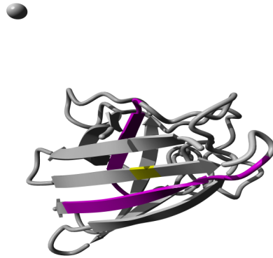
Figure 2.12: Molecular visualisation of LIMBO chaperone-binding sites. This molecular image shows the LIMBO chaperone-binding sites as pink colored segments. The structural location of the variant residue is colored in yellow.
