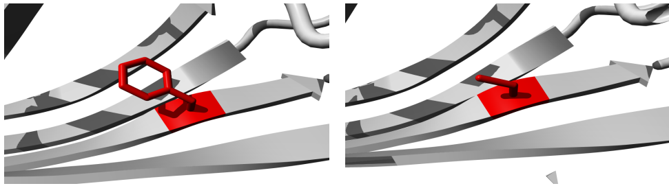
Figure 2.13: Molecular visualization of the WT (left) and variant (right) amino acid. The residues colored in red represents the wild type (PHE) and variant residue (CYS).
