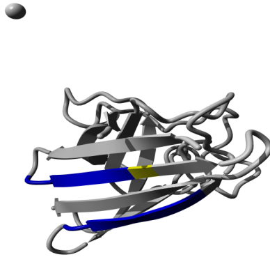
Figure 2.8: Molecular visualisation of WALTZ amyloid-forming regions. This molecular image shows the WALTZ aggregation-prone regions as blue colored segments. The structural location of the variant residue is colored in yellow.
