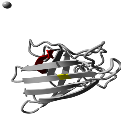
Figure 2.4: Molecular visualisation of TANGO aggregation-prone regions. This molecular image shows the TANGO aggregation-prone regions as red colored segments. The structural location of the variant residue is colored in yellow.
