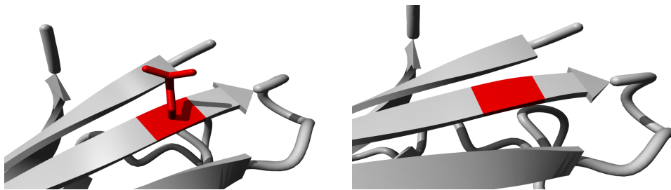
Figure 2.13: Molecular visualization of the WT (left) and variant (right) amino acid. The residues colored in red represents the wild type (GLU) and variant residue (GLY).
