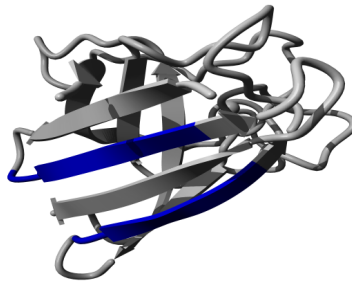
Figure 2.8: Molecular visualisation of WALTZ amyloid-forming regions. This molecular image shows the WALTZ aggregation-prone regions as blue colored segments. The structural location of the variant residue is colored in yellow.
