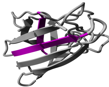
Figure 2.12: Molecular visualisation of LIMBO chaperone-binding sites. This molecular image shows the LIMBO chaperone-binding sites as pink colored segments. The structural location of the variant residue is colored in yellow.
