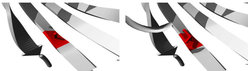
Figure 2.13: Molecular visualization of the WT (left) and variant (right) amino acid. The residues colored in red represent the wild type (ALA) and variant residue (VAL).
