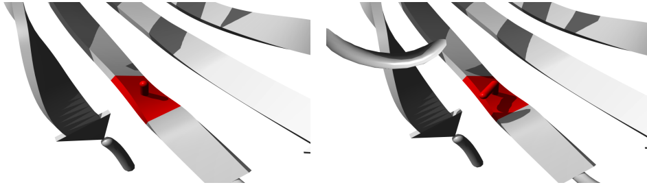
Figure 2.13: Molecular visualization of the WT (left) and variant (right) amino acid. The residues colored in red represents the wild type (ALA) and variant residue (SER).
